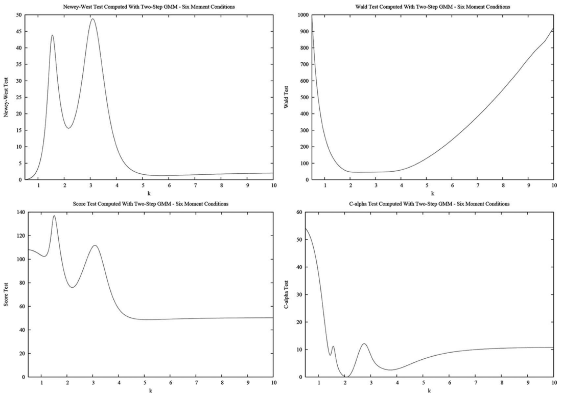
Figure 2. Two-step GMM tests based on six moment conditions.
