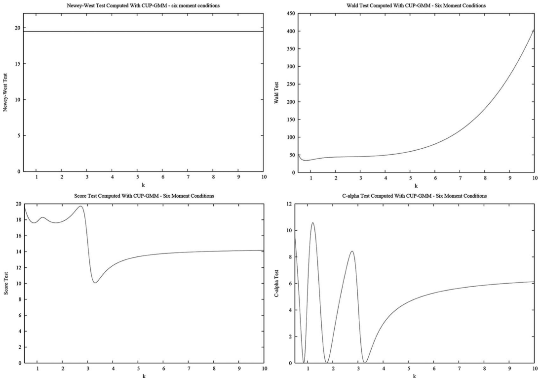
Figure 3. CUP GMM tests based on six moment conditions.
