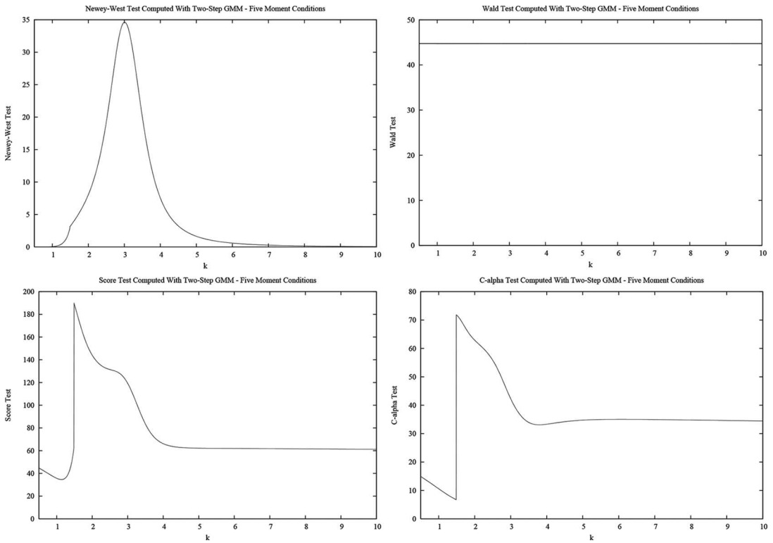
Figure 1. Two-step GMM tests based on five moment conditions.
